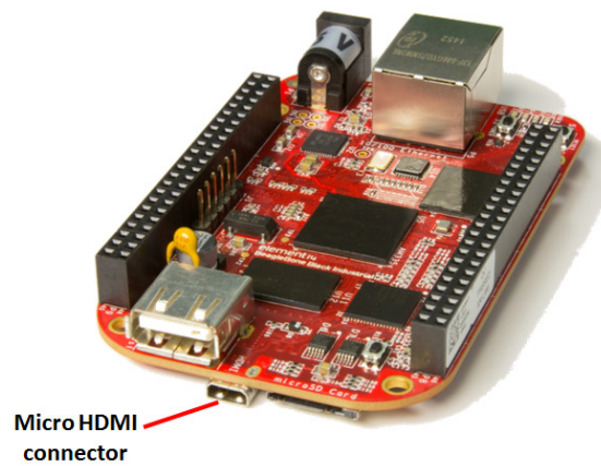
Figure 57 HDMI Connector
