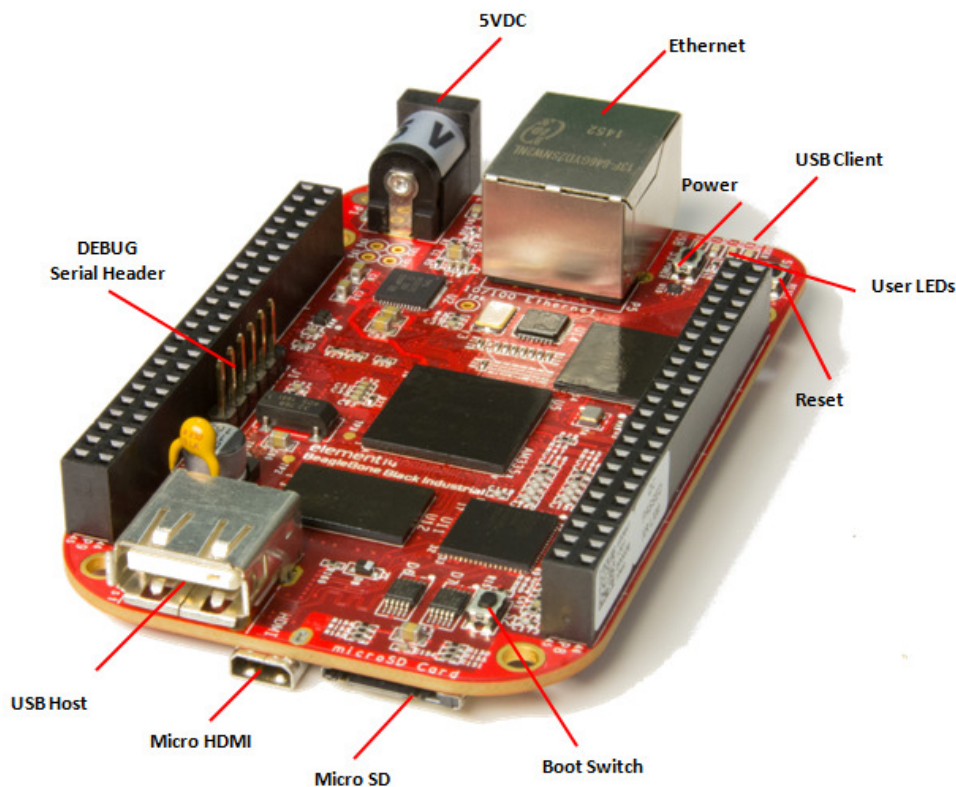
Figure 17 Connectors, LEDs and Switches
