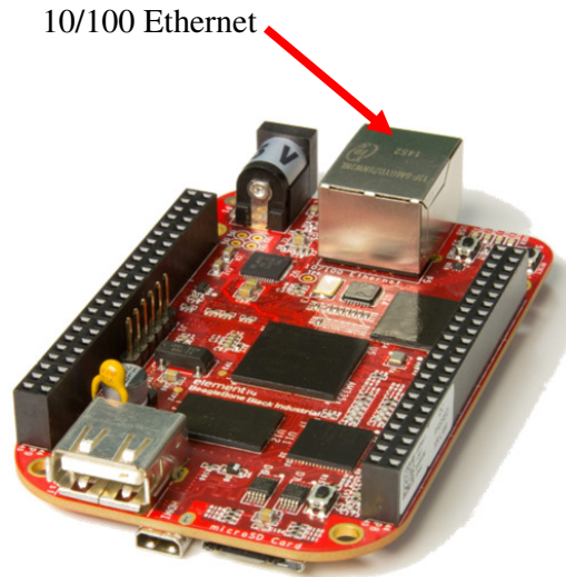
Figure 60 Ethernet Connector
