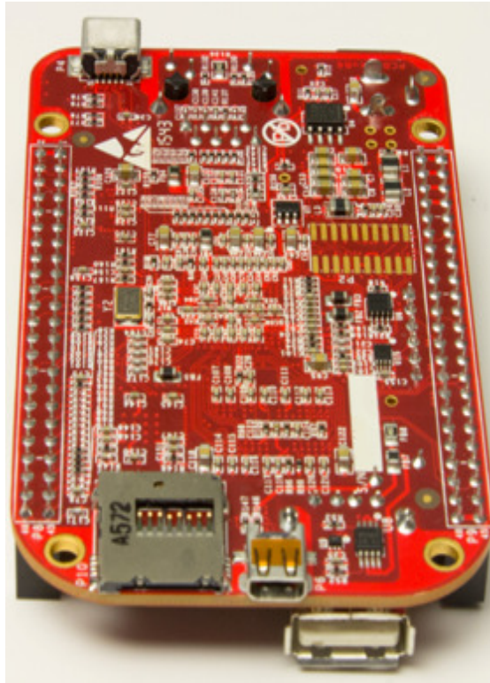
Figure 75 Bottom Side
