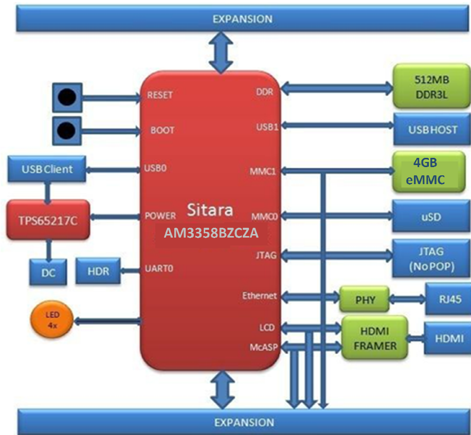
Figure 20 element14 BeagleBone Black Industrial Block Diagram
