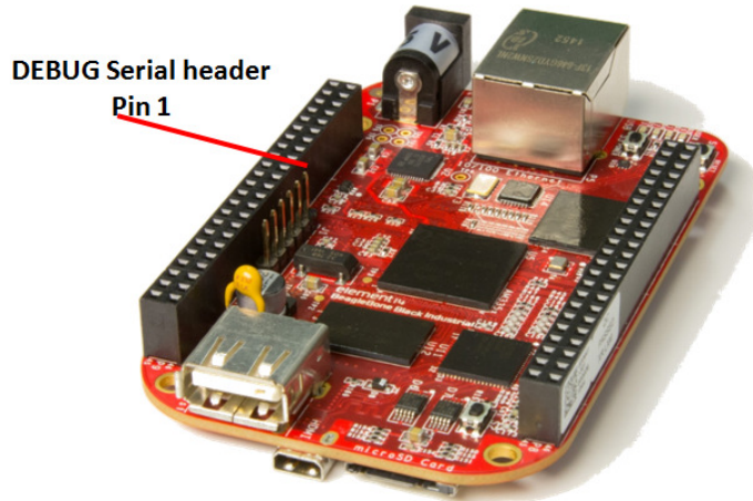
Figure 54 Serial Debug Header
