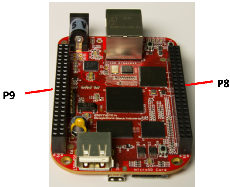
Figure 50 Expansion Connector Location
