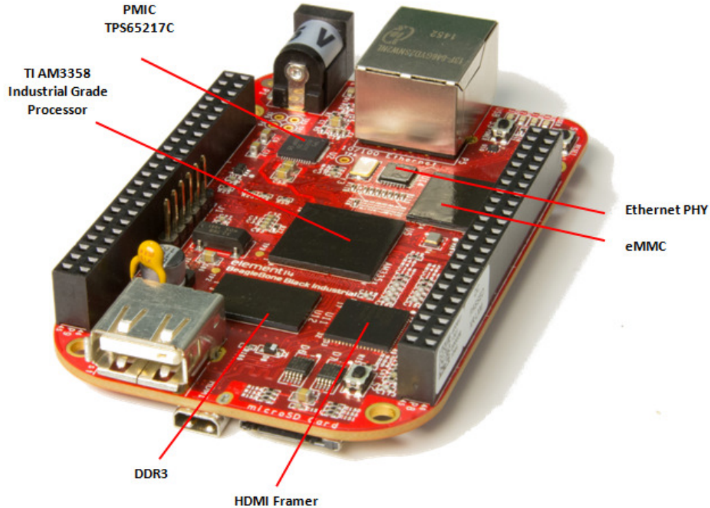
Figure 18 Key Components
