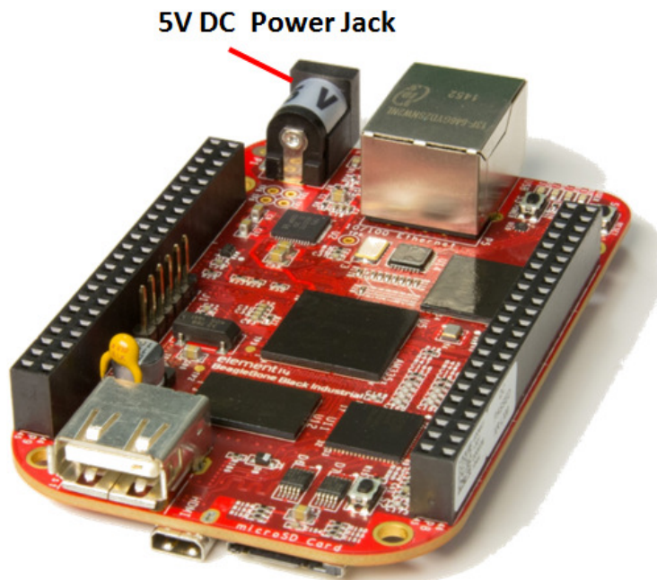
Figure 51 5VDC Power Jack
