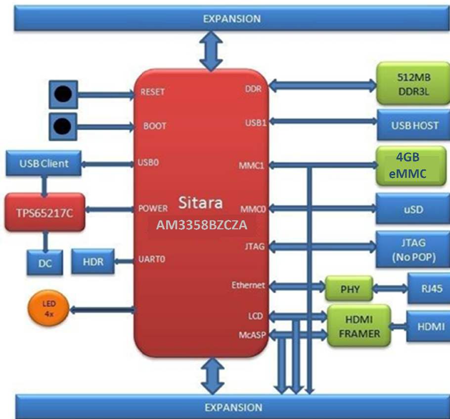
Figure 19 element14 BeagleBone Black Industrial Key Components
